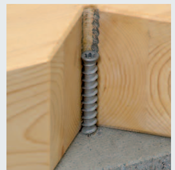
MULTI-MONTI®-TimberConnect
